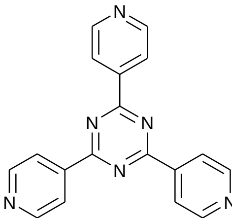
2,4,6-tris(4-pyridyl)-1,3,5-triazine tpt
