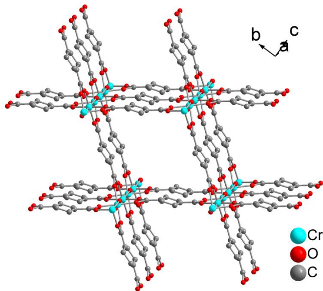
3D network
